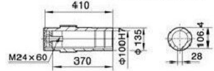
FA127/FAF127/FAZ127空心轴 /Hollow shaft
